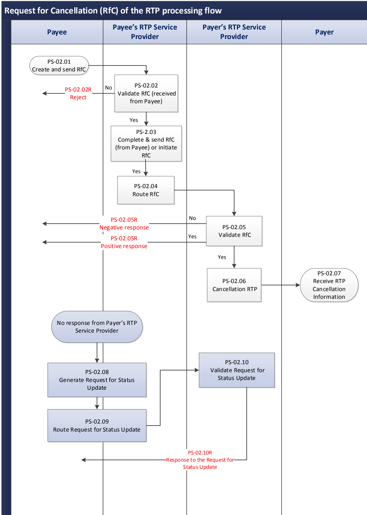
Figure 6: RfC of the RTP – processing flow (PS-02)
