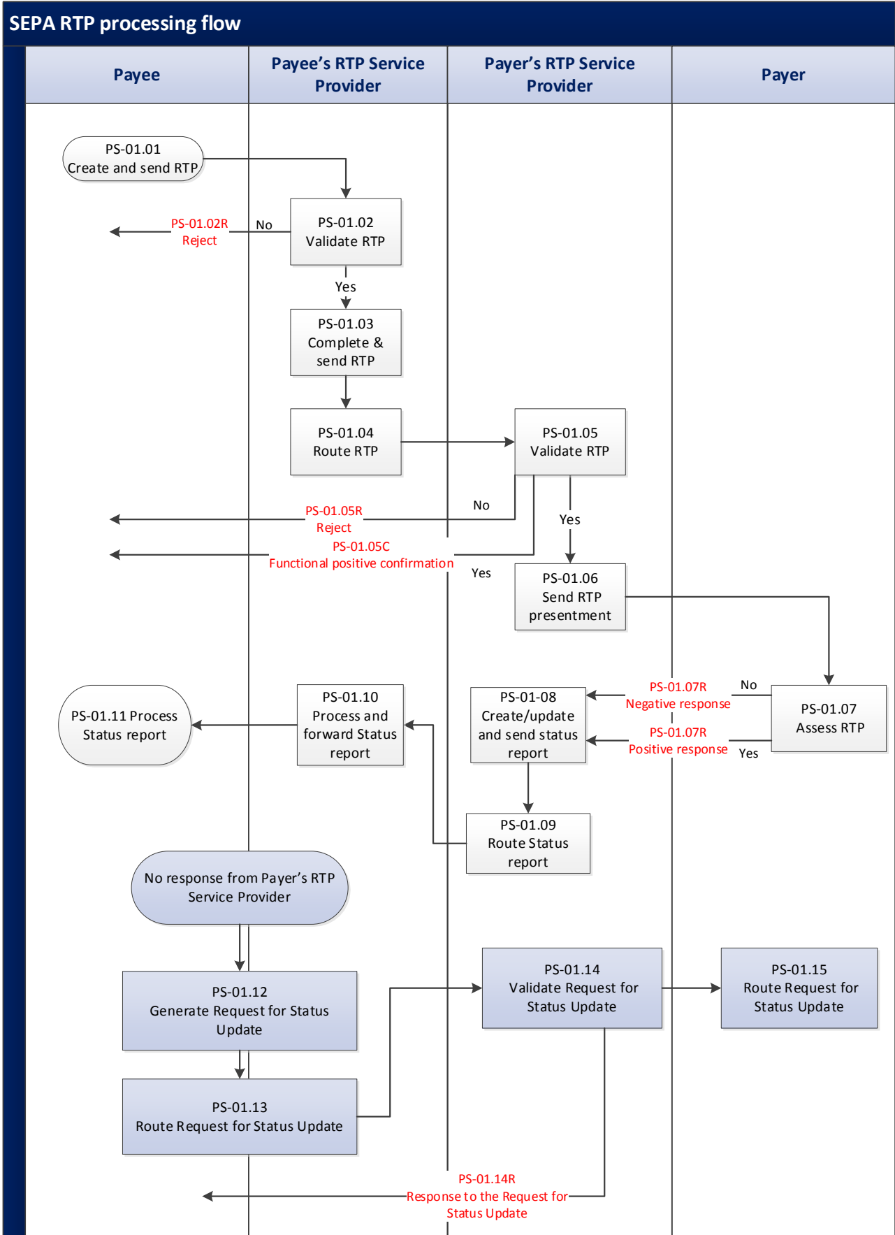
Figure 5: RTP Processing flow (PS-01)
